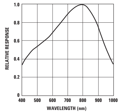
Figure 16. Wavelength Responsivity [1] .
