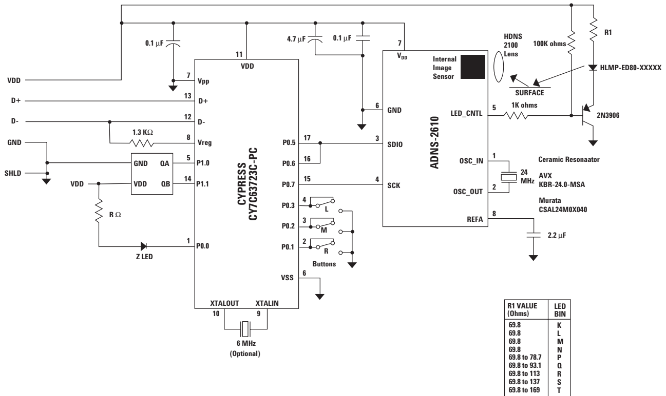
Figure 8. Circuit block diagram for a typical corded optical mouse using an Agilent ADNS-2610 optical mouse sensor.
