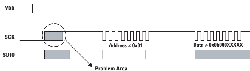
Figure 28. Power-up serial port sequence.
